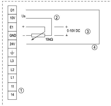
External speedsetting
