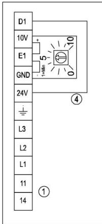
Internal potentiometer
