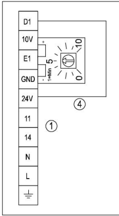
Internal potentiometer
